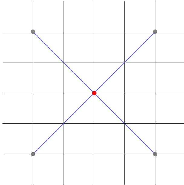
Figure 347: How the diamond-square algorithm works (2/5)
